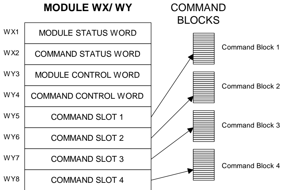
Figure 7. PLC Command Interface
